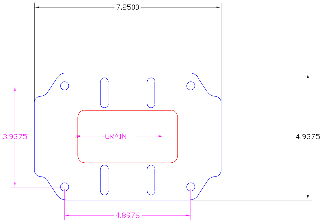
PC680 universal batt mount base plate
