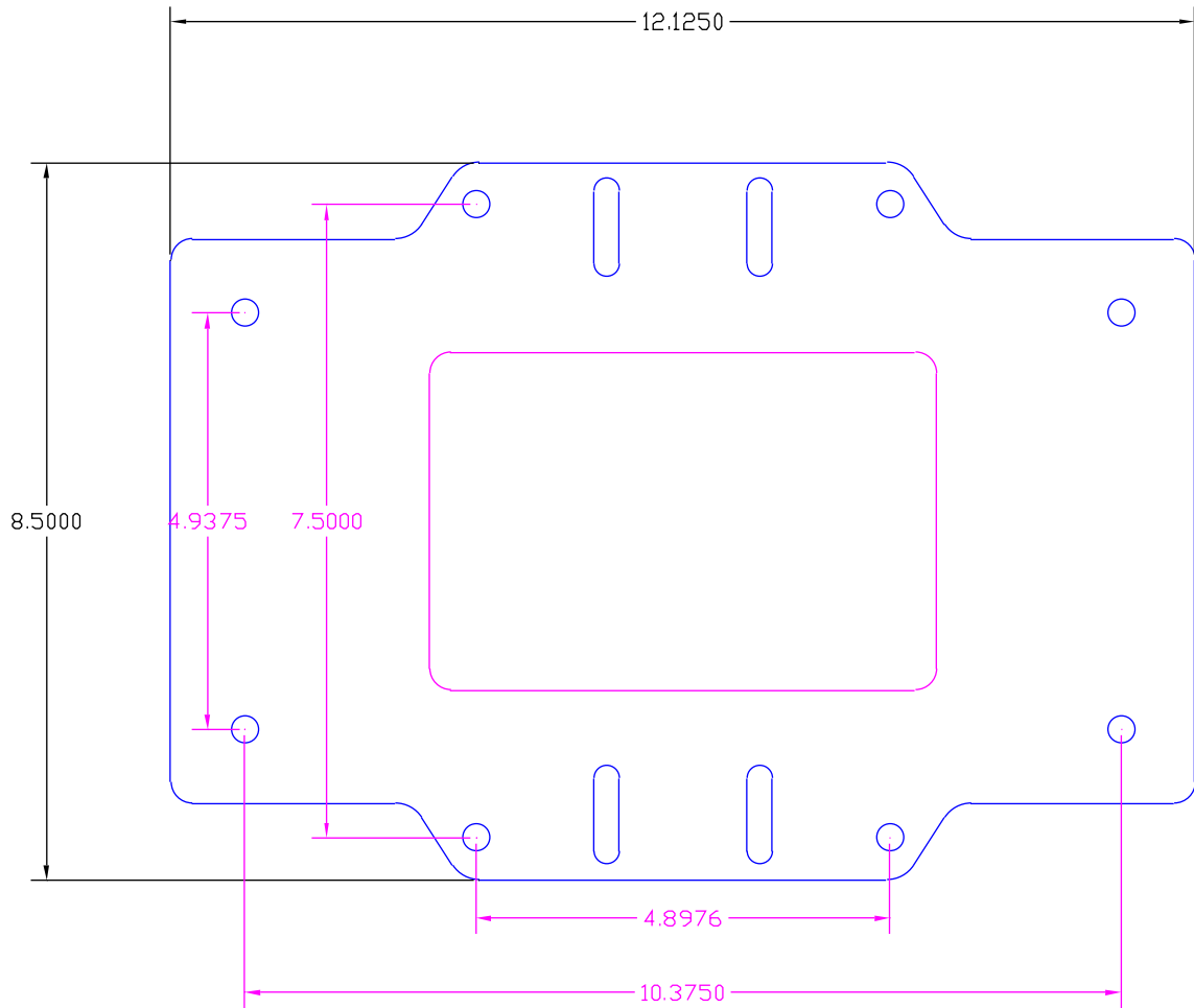
PC1700 universal kit battery mount base plate
