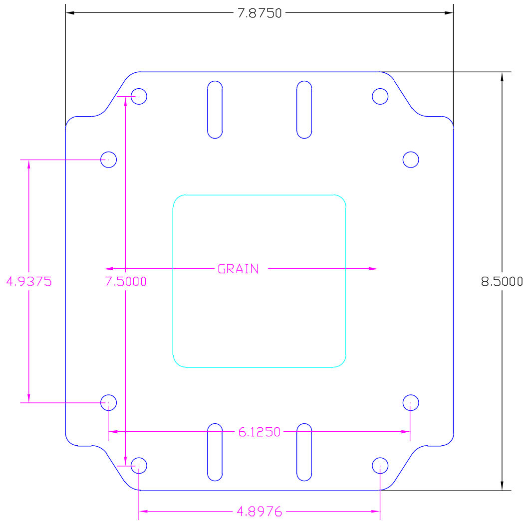
PC1200 universal battery mount base
